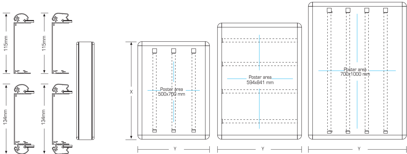
LIGHT BOX EXTRUSION AND LIGHT BOX ROUNDS DESIGNED BY ORES, JANUARY 1997
